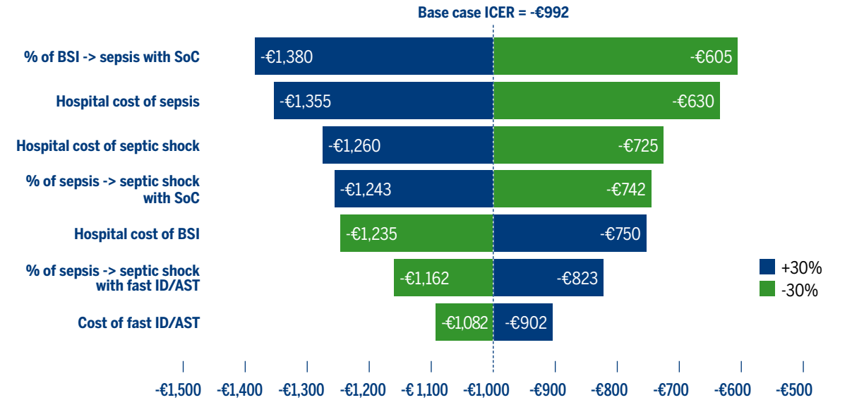
Figure 1. Tornado diagram – net cost savings per patient when +/- 30% variation is applied for each variable Reproduced with permission from Boughazi HE.
