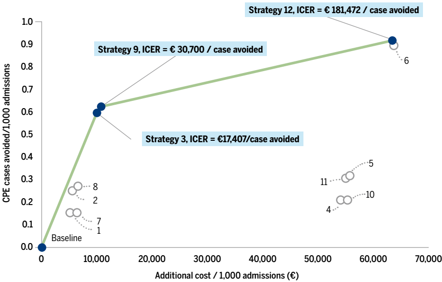
Figure 1. Cost-effectiveness plane showing incremental benefits and costs relative to the least expensive strategy (baseline) Reproduced with permission from Kardas-Sloma et al. Antimicrobial Resistance and Infection Control 2022;11:117
